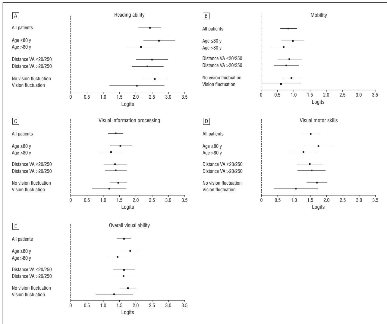
Figure 2. Differences in mean changes in reading ability (A), mobility (B), visual information processing (C), visual motor skills (D), and overall visual ability (E) for all patients and within subgroups of patients defined by age, baseline distance visual acuity, and presence or absence of visual fluctuations. The data points represent differences in mean 4-month changes between the treatment and control groups. All patients: n=126; age ≤80 y: n=61; age >80 y: n=65; distance VA ≤20/250: n=66; distance VA >20/250: n=60; no vision fluctuation: n=96; vision fluctuation: n=30. VA indicates visual acuity.
